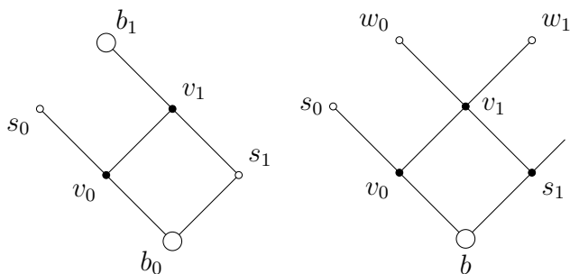
Fig. 1. The forbidden configurations of Lemma 2.4 and Lemma 2.5. The big vertices are represented with big circles, and the small vertices with small circles. The filled circles represent vertices whose incident edges are all represented.
